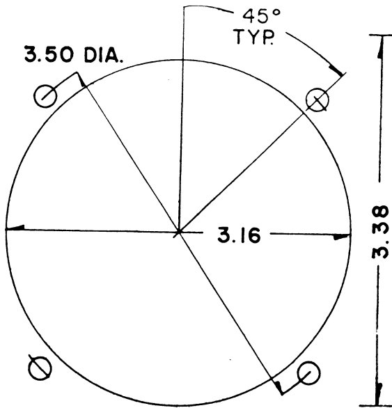
TYPICAL CUT-OUT MOST STANDARD INSTRUMENTS (AIR SPEED, 3-IN-1 GAUGE, COMPASS)
