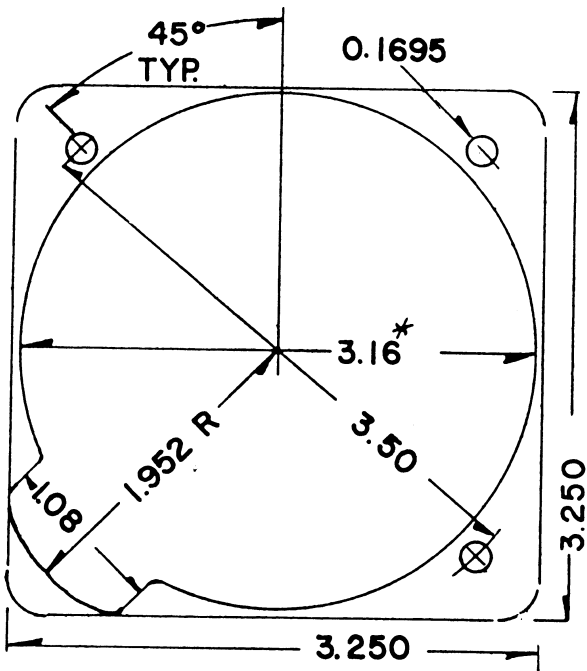
TYPICAL CUT-OUT (MOST ALTIMETERS, RATE-OF-CLIMB, LARGE MANIFOLD PRESSURE)
