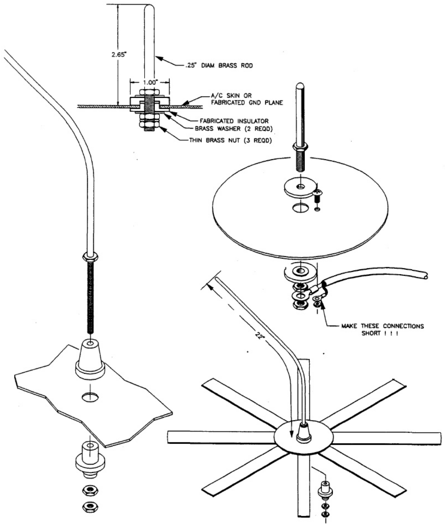
Figure 13-8. Variations on the Quarter-Wave Ground Plane.
