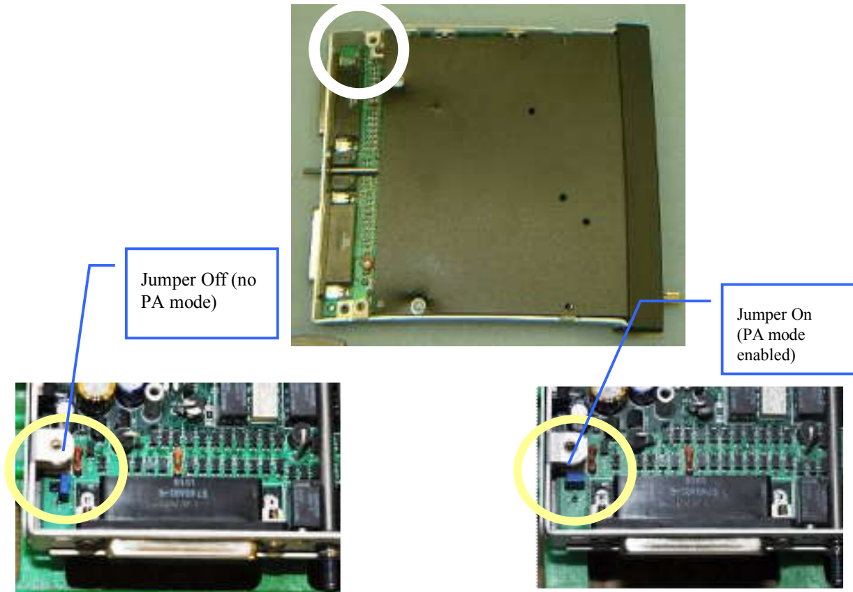
Figure 2-3 Jumper Location
