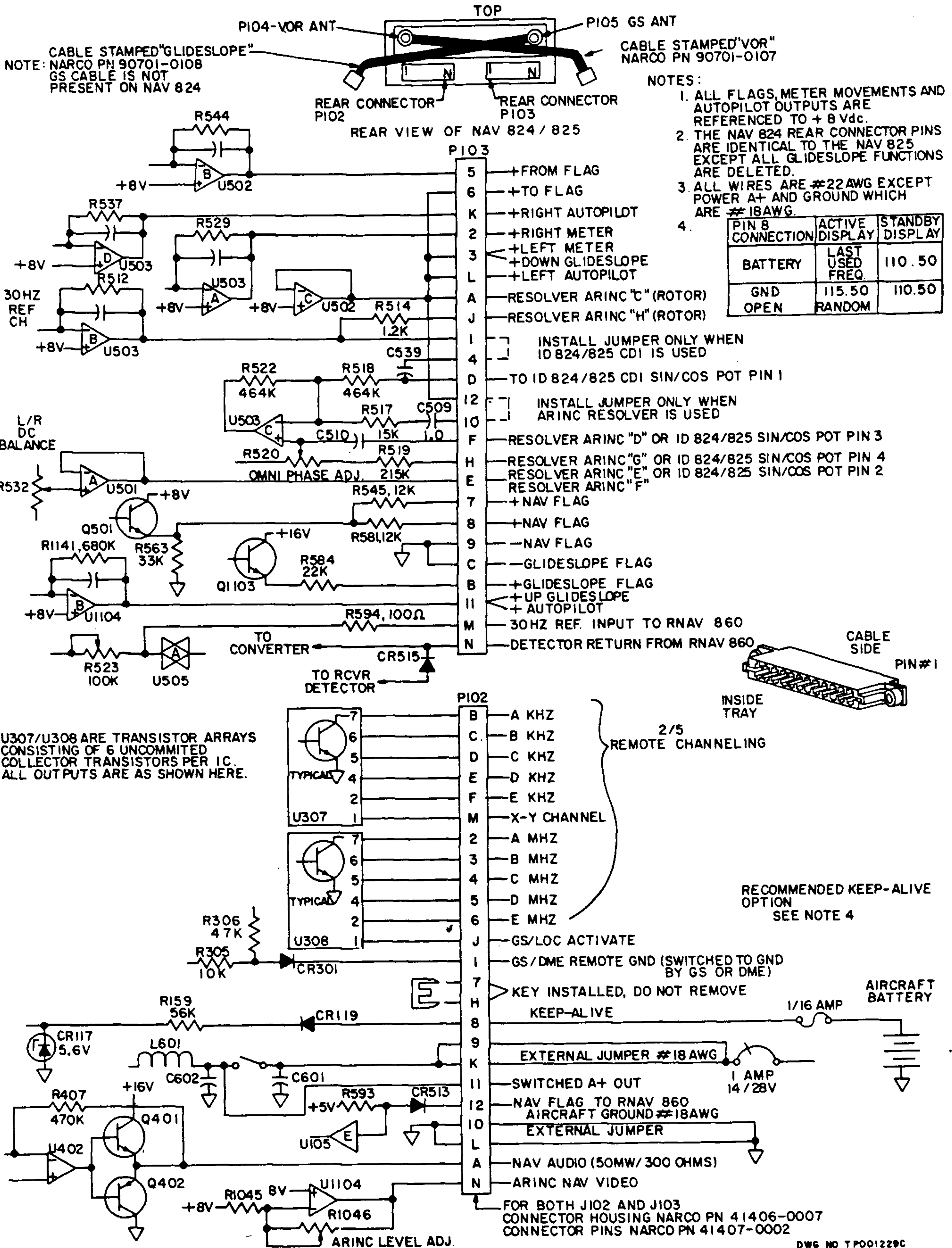
FIGURE 2-6. INTERCONNECT WIRING, NAV 824/825
