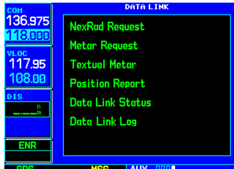
Figure 5-23. Data Link Page
