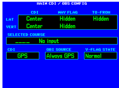
Figure 5-11. MAIN CDI/OBS CONFIG Page
