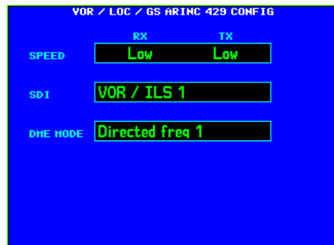
Figure 5-15. VOR/LOC/GS ARINC 429 CONFIG Page
