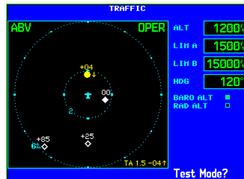
Figure 5-19. TRAFFIC Page (Skywatch)
