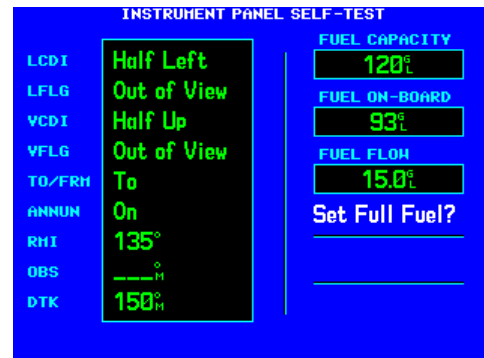
Figure 5-6. INSTRUMENT PANEL SELF-TEST Page
