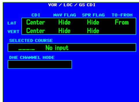
Figure 5-14. VOR/LOC/GS CDI Page
