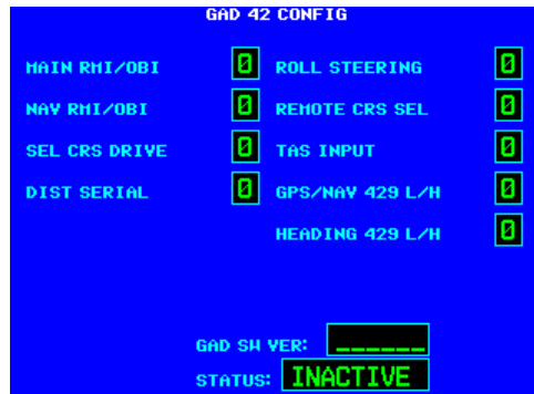
Figure 5-22. GAD 42 CONFIG Page
