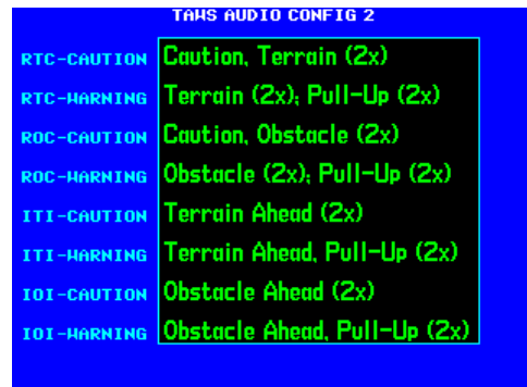
Figure 5-25. TAWS AUDIO CONFIG Page 2
