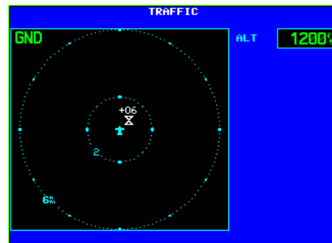
Figure 5-20. TRAFFIC Page (TCAD)
